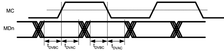
FIGURE 1. Serial Data Valid — SLV Input Set and Hold Time
