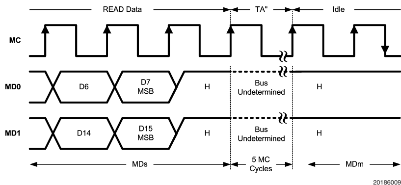
FIGURE 10. READ_Data and TA''
