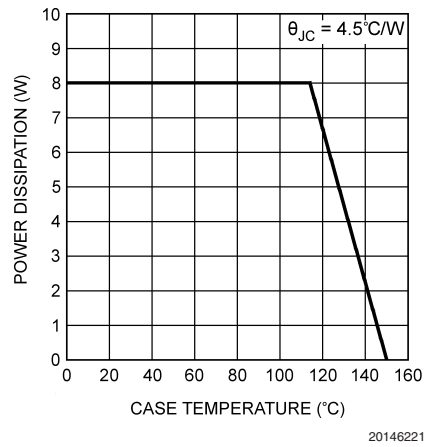
FIGURE 10. Power Derating Curve
