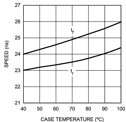
FIGURE 8. Speed vs Case Temperature
