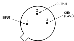
Steel Metal Can TO-39 Package (H)
