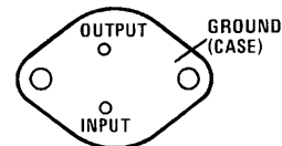
TO-3 Metal Can (K)
