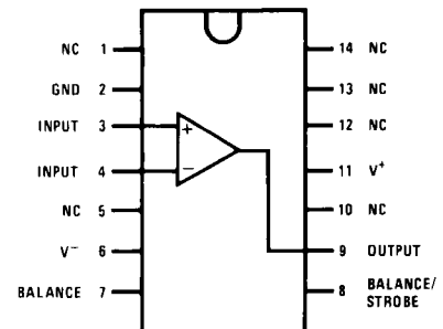
Dual-In-Line Package
