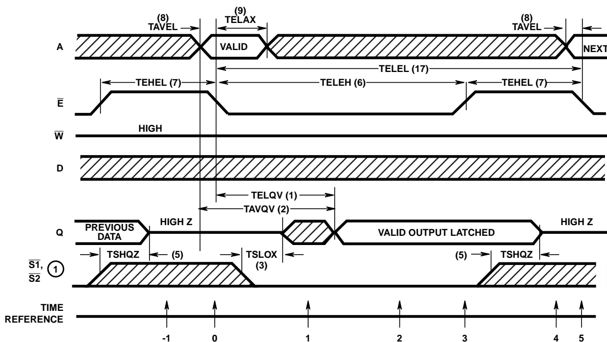
FIGURE 1. READ CYCLE
