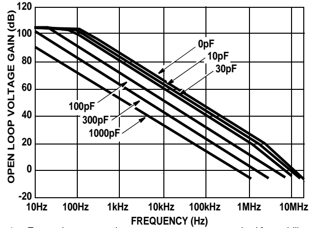
FIGURE 14. OPEN LOOP FREQUENCY RESPONSE FOR VARIOUS VALUES OF CAPACITORS FROM COMPENSATION PIN TO GROUND
