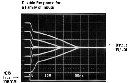
A_V = +2 , R_L = 150\Omega , V_S = \pm 5V
