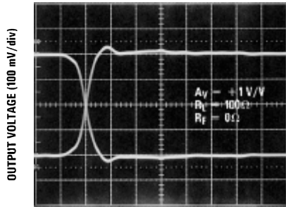
TIME (2 ns/div)
