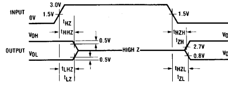
FIGURE 12. Waveform
