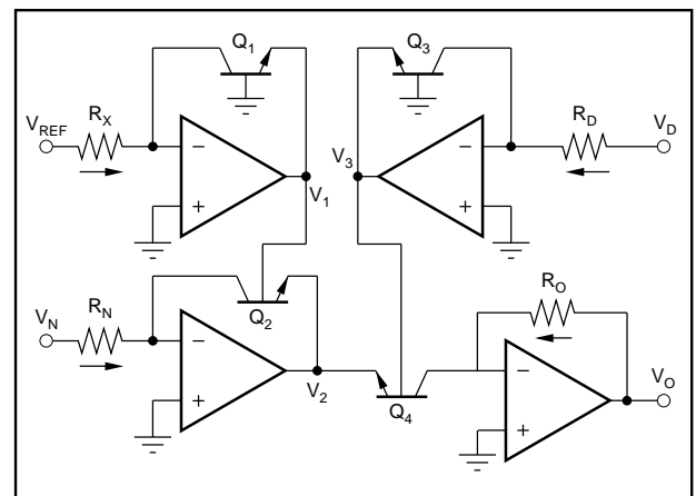
FIGURE 4. One-Quadrant Log-Antilog Divider.
