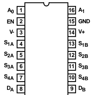
DG509A (PDIP, SOIC) TOP VIEW
