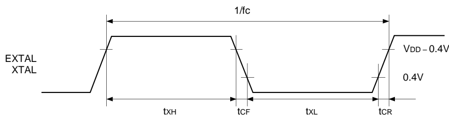
Fig. 1. Clock timing
