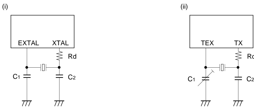
Fig. 13. Recommended oscillation circuit
