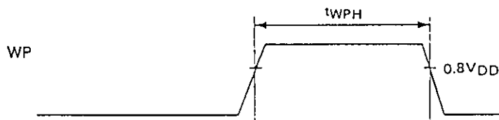
Fig. 8. Wake-up input timing
