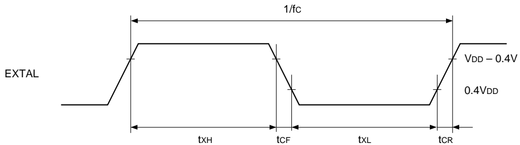
Fig. 1. Clock timing
