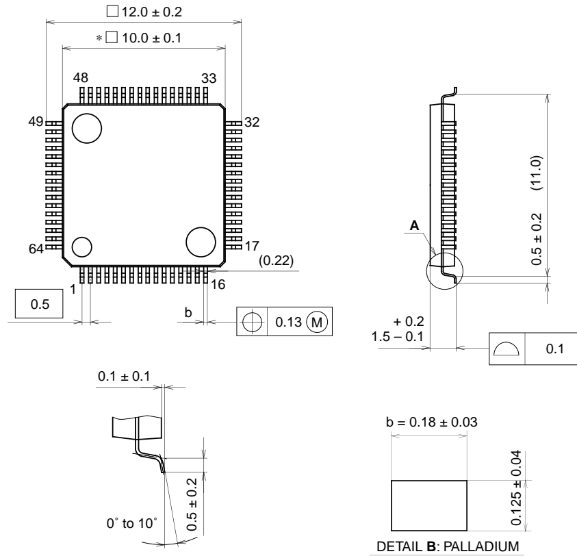
DETAIL A
