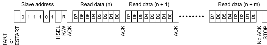
Continuous Read Operation
