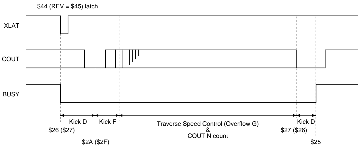
Fig. 4-12 (b). Fine Search Timing Chart
