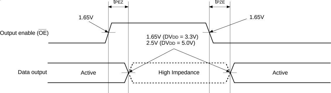
Timing Chart 2
