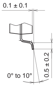
DETAIL A
