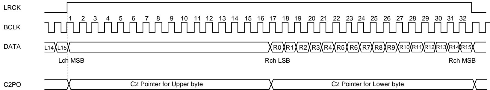
Fig. 2.1.1 (4) CXD2500Q, 64 bit Slot Mode Timing Chart
