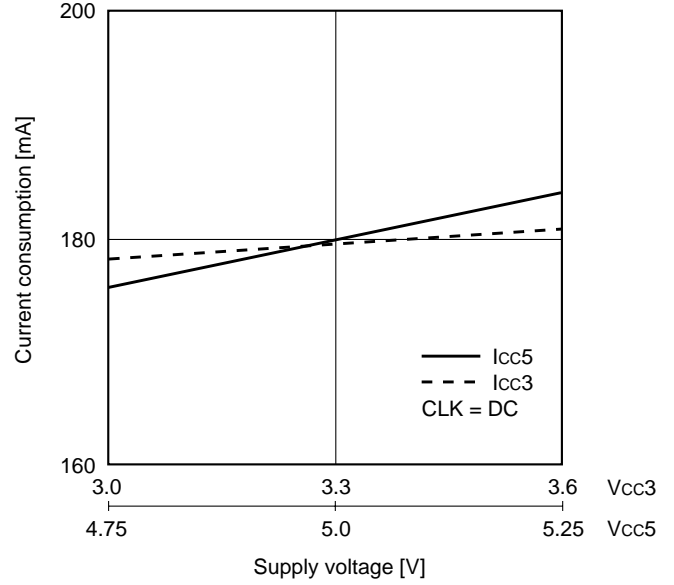
Current Consumption vs. Supply Voltage Fluctuation
