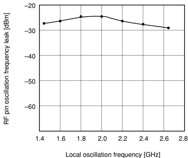
RF pin oscillation frequency leak vs. Local oscillation frequency
