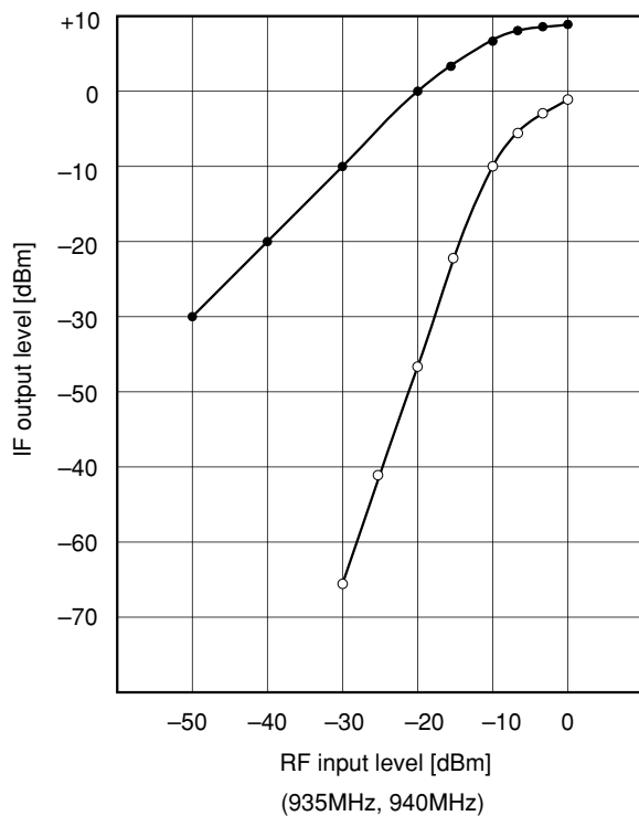
Input/output characteristics (untuned input)
