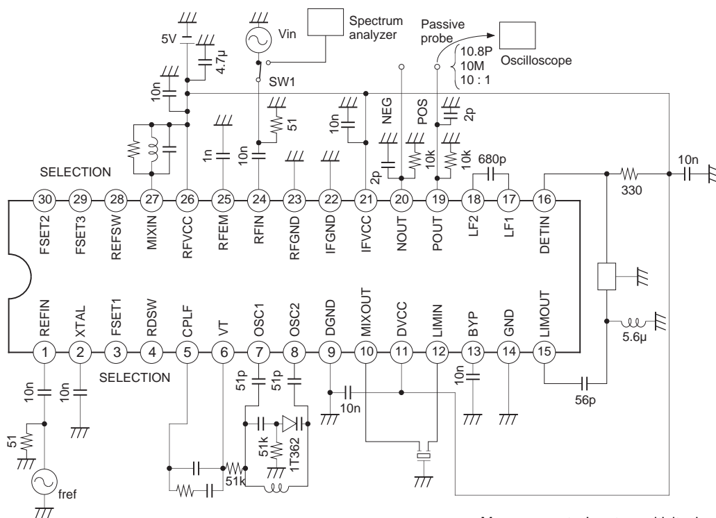
Measurement : Input sensitivity, local osc leakage, FSK DATA output voltage, rise time, fall time
