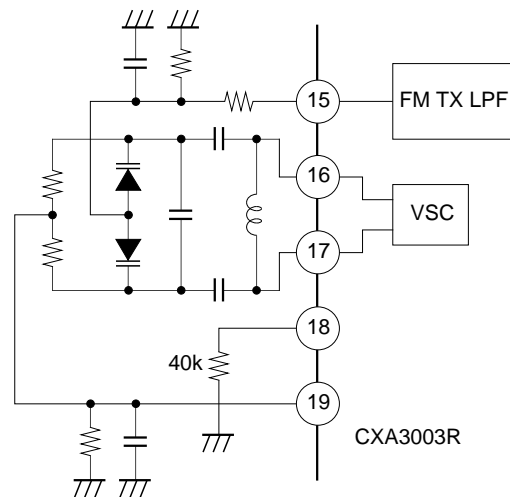
Fig. 12 Transmit VCO
