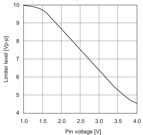
Black level limiter adjustment characteristics
