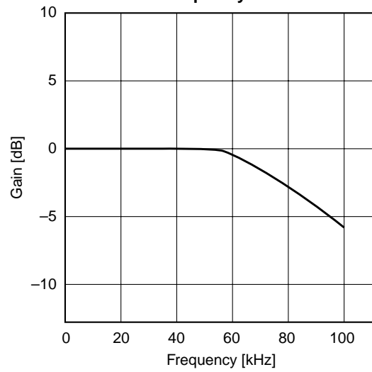
Main LPF and Sub LPF frequency characteristics
