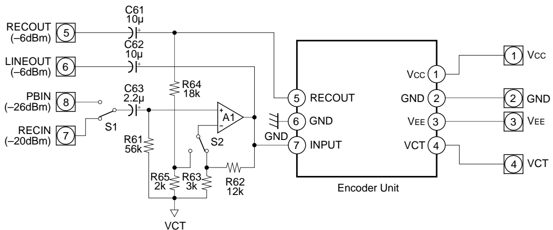
Fig. 3. Switchable Processor
