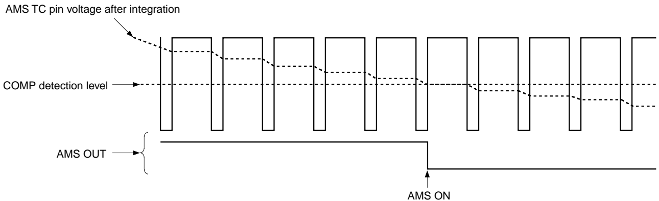
Fig. 6. Conceptual diagram of AMS OUT operation
