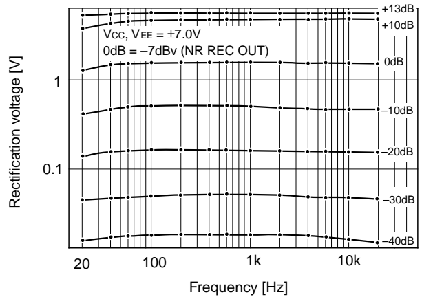
Playback equalizer amplifier distortion
