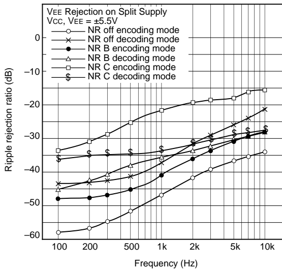
NR ripple rejection ratio 2
