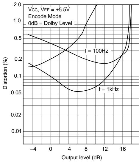
NR C type total harmonic distortion
