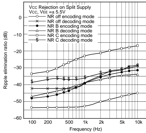
NR ripple rejection ratio 1
