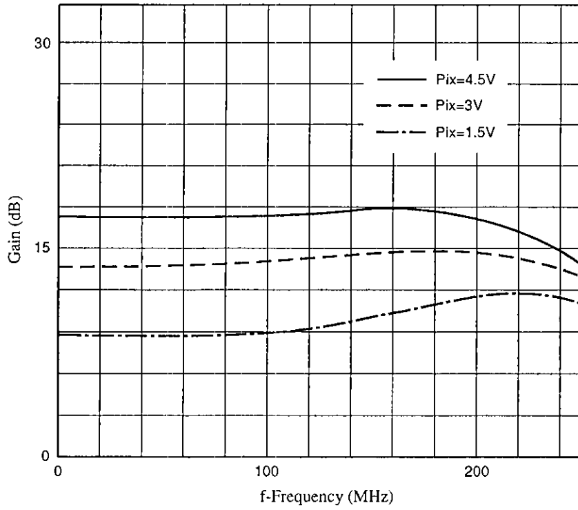
Frequency response
