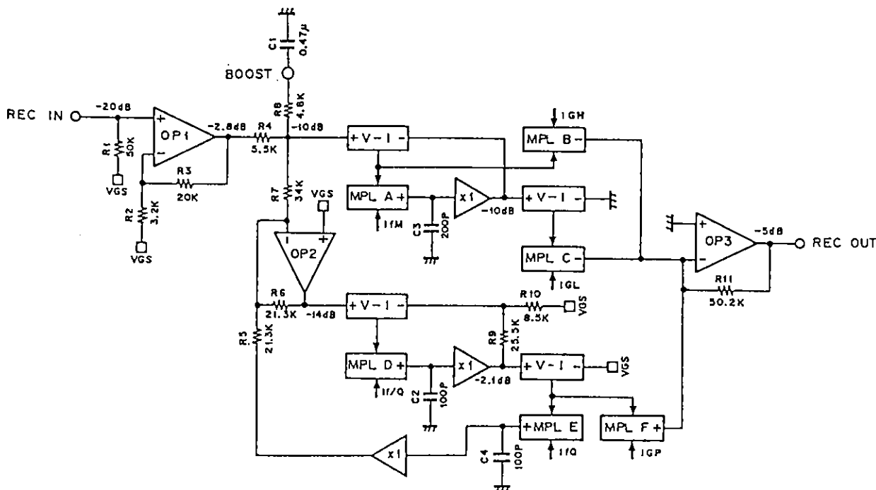
Fig. 1. CXA1579 functional circuit block diagram
