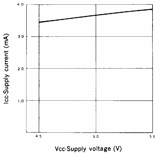
Supply current vs. Supply voltage ( SW=MOD= \text{High} , T_a=25^\circ\text{C} )
