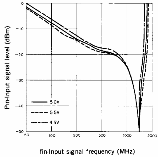
Input Signal Level vs. Operating Frequency Characteristics 2 T_a=25^\circ\text{C}
