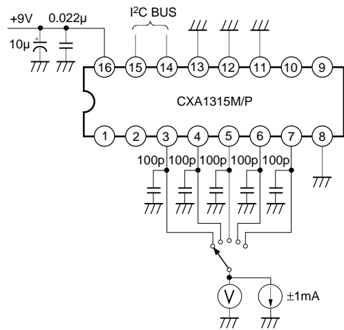
Measurement Circuit 2
