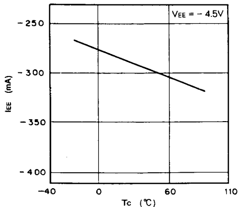
Power supply current vs. T_c
