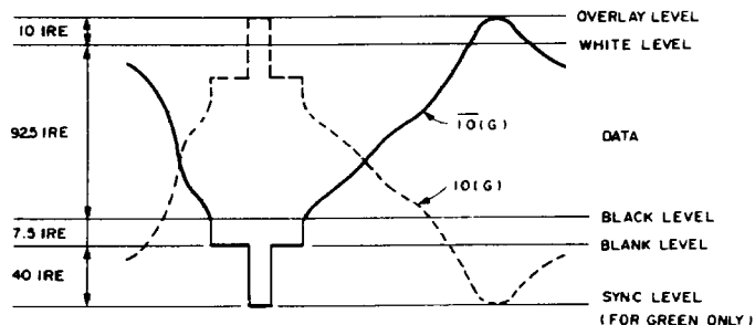
Fig. 1. Composite Video Output Level (GREEN)
