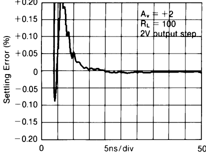
Settling Time
