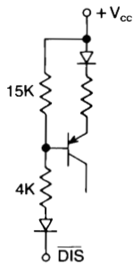
Figure 4: equivalent of \overline{\text{DIS}} input
