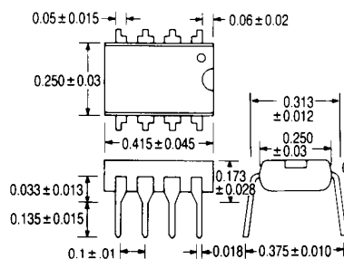
8-pin Plastic DIP
