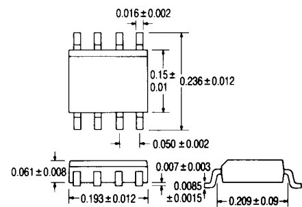
8-pin Plastic SOIC
