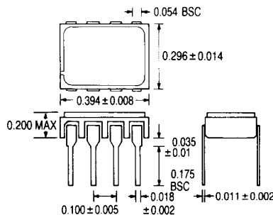
8-pin Side-brazed Ceramic DIP
