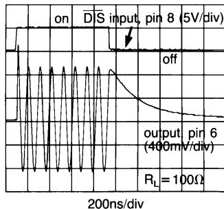
Enable/Disable Response
