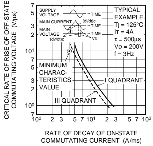
COMMUTATION CHARACTERISTICS
