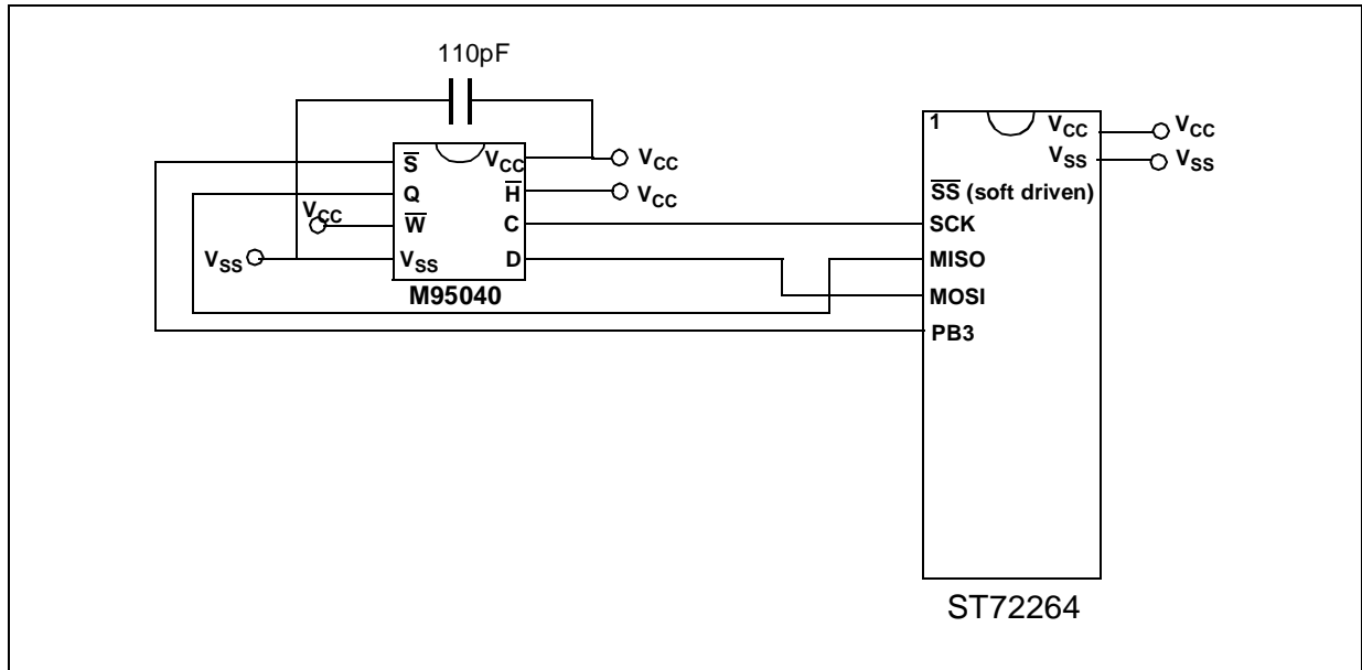
Figure 2. Hardware description
