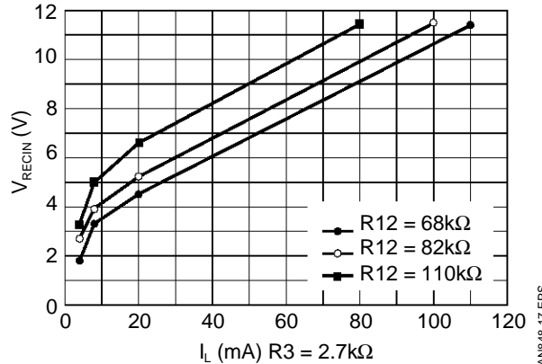
Figure 18 : V_{RECIN} (Pin 19)
