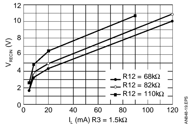
Figure 18 : V_{RECIN} (Pin 19)
