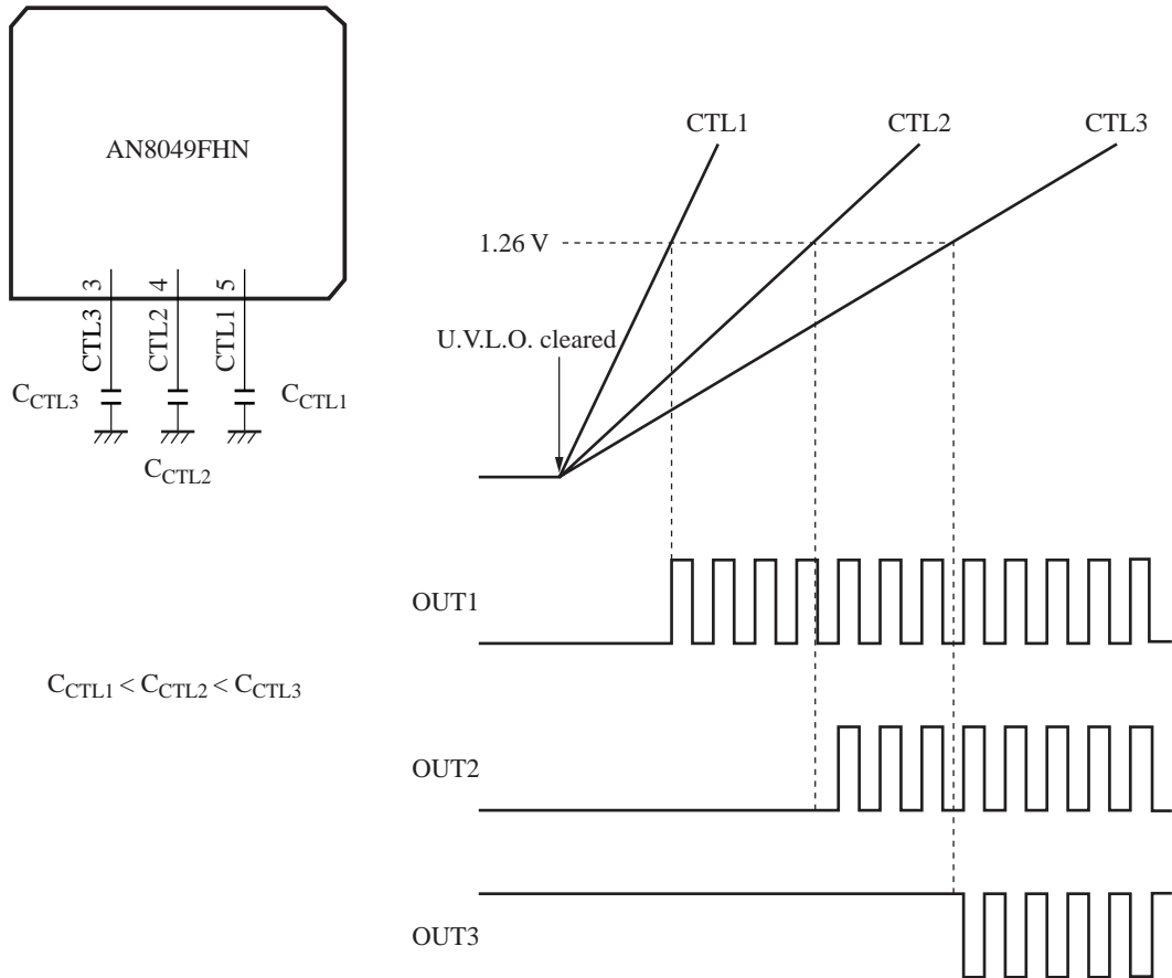
Figure 8. Sequential operation
