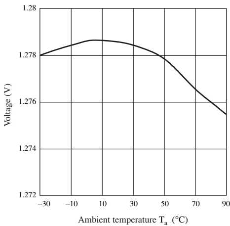
Error amplifier V_{TH} temperature characteristics
