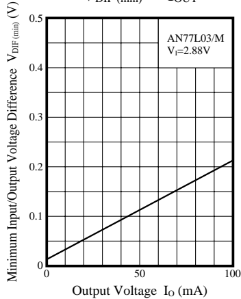
Minimum Input/Output Voltage Difference V_{\text{DIF}(\text{min})} - I_{\text{OUT}}
