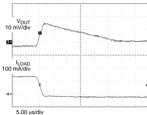
Figure 5. Load Transient Response-1
