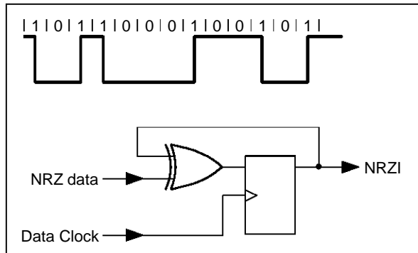
Figure 15 : NRZI code
