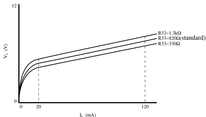
Fig.1—3 I_L-V_L Characteristics
