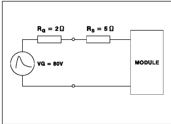
Figure 7 : Application Diagram
