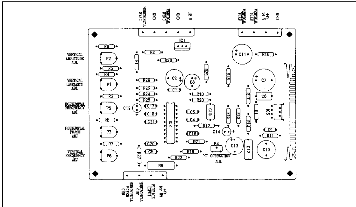
Figure 20 : PCB Layout
