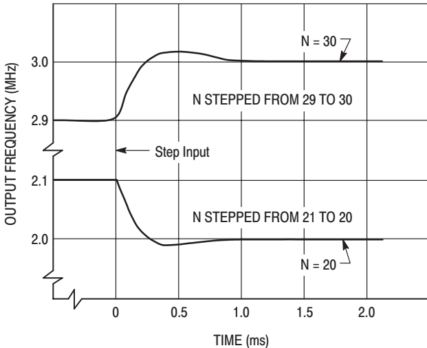
Figure 13. Frequency-Time Response
