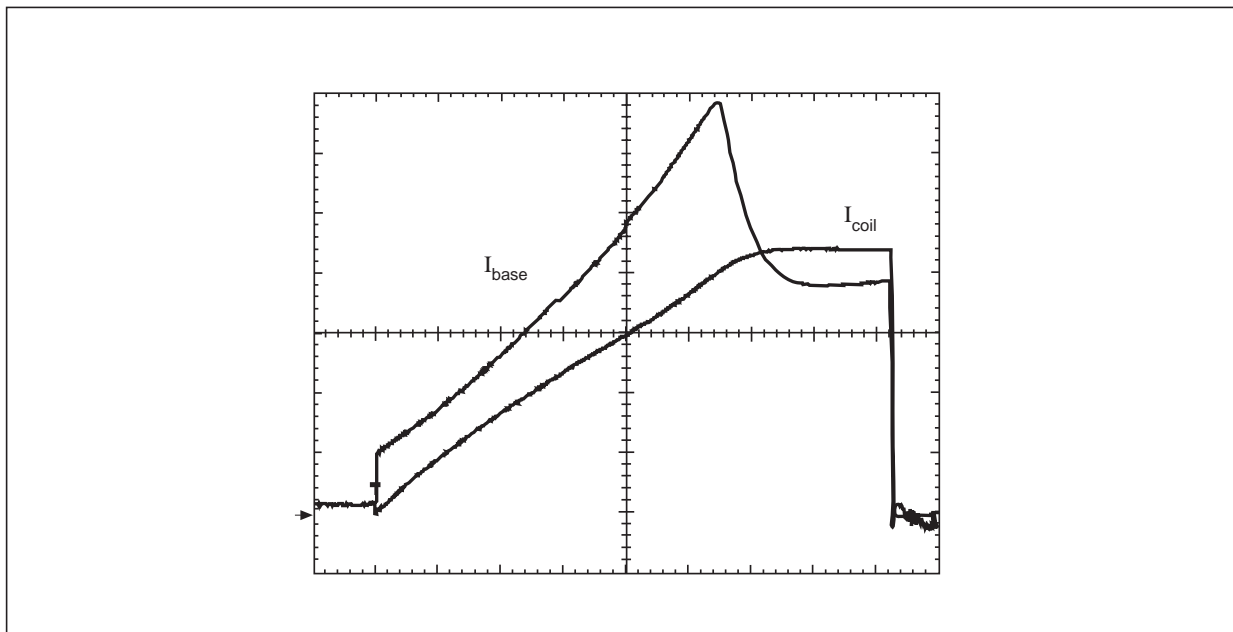
Figure 5. Base driver operation
