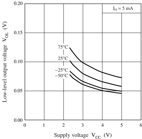
Low-level output voltage — Supply voltage
