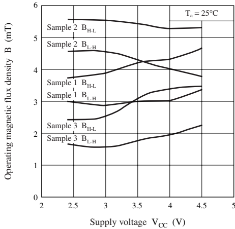
Operating magnetic flux density — Supply voltage
